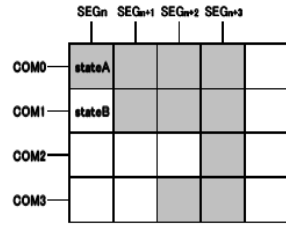
(1/2bias) LINE 翻转
