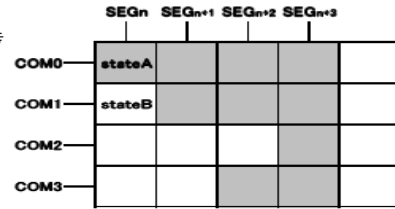
(1/3bias) FRAME 翻转
