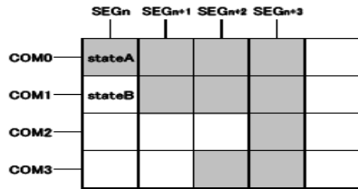
(1/3bias) LINE 翻转
